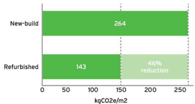
Figure 1. Embodied carbon emissions of an 8-bay modular building
